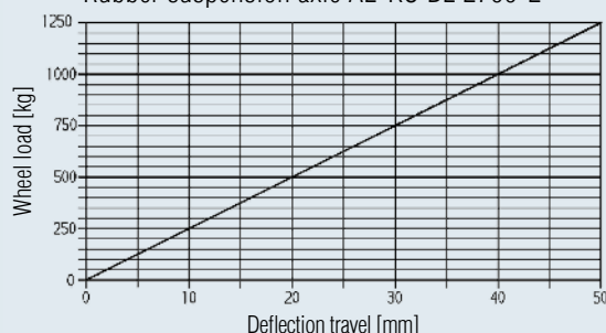
Rubber suspension axle AL-KO BL 2700-2
