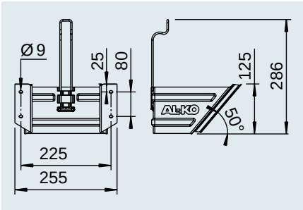
Holder HA 53 St for UK 53 steel and plastic
