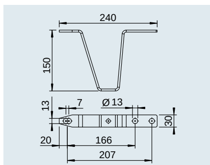
Skid bracket (bottom installation) for overrun device Profi 3000/3500
