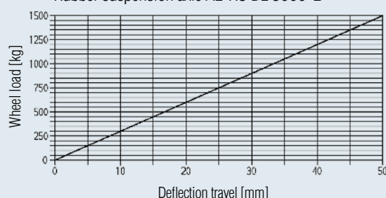
Rubber suspension axle AL-KO BL 3000-2
