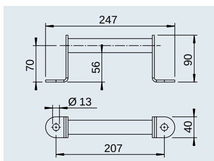
Manoeuvring handle for overrun device Profi 3500
