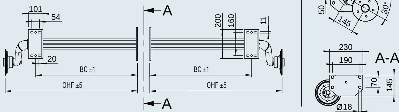
Part No. 1426205
