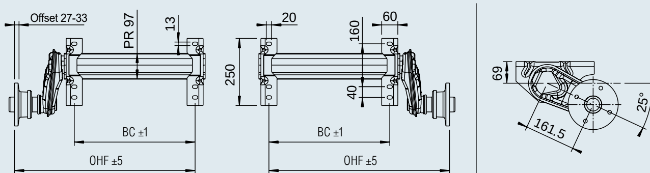
Part No. 1421391
