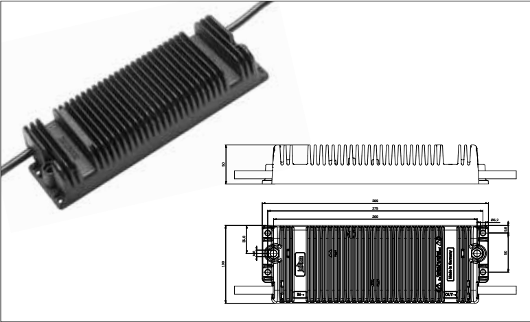
LED controller "LK 2000-1"
