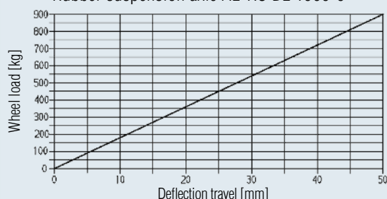
Rubber suspension axle AL-KO BL 1900-9
