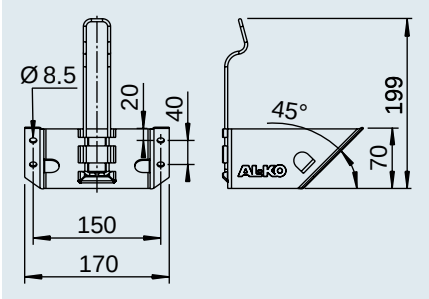
Holder HA 36 St for UK 36 steel and plastic
