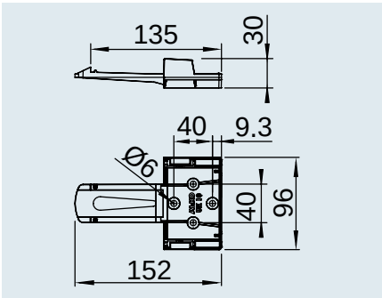
Holder HA 10 K-2 for UK 10 K-2
