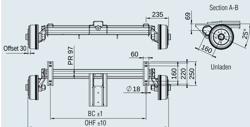
Axle with slave cylinder attachment kit cpl. (special variant) B 1800
