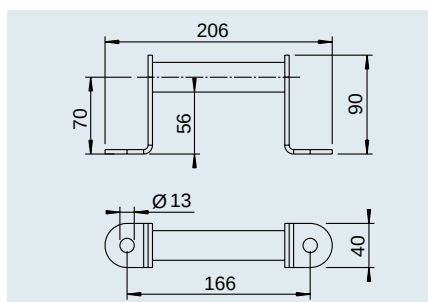
Manoeuvring handle for overrun device Profi 3000
