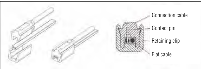
Snap-in retaining clip
