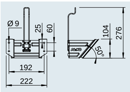
Holder HA 46 St for UK 46 steel and plastic
