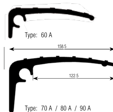
Supporting profile "B"
