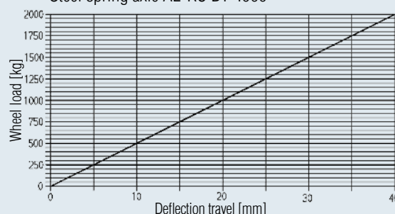
Steel spring axle AL-KO BT 4000
